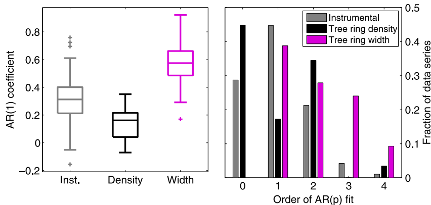
Fig. 3. Left panel: box plots of AR(1) coefficients inferred from the instrumental, tree ring density, and tree ring width time series depicted in Figs. 1 and 2. Results are not shown for the ice core and lake data sets due to the small number of series. Right panel: optimal order of AR(p) fit, according to the Bayesian Information Criterion (analysis performed with the ARFit Matlab package described in Neumaier and Schneider (2001) and Schneider and Neumaier (2001)).
